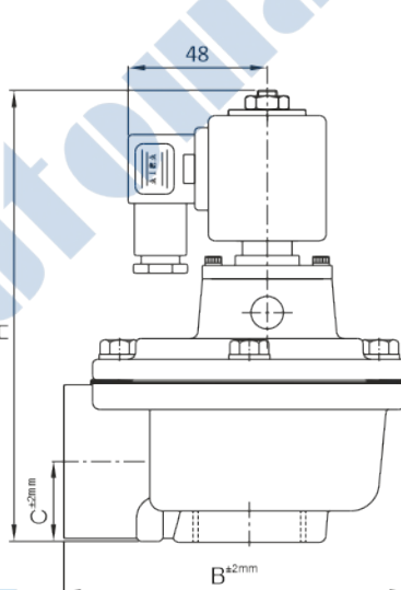
Explosion & Flame Proof Coil [As per IS / IEC 60079-1 standard approved by Central Institute of Mining and Fuel Research (CIMFR)]
