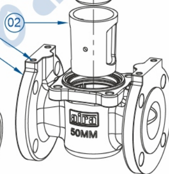
Flanged End Body
